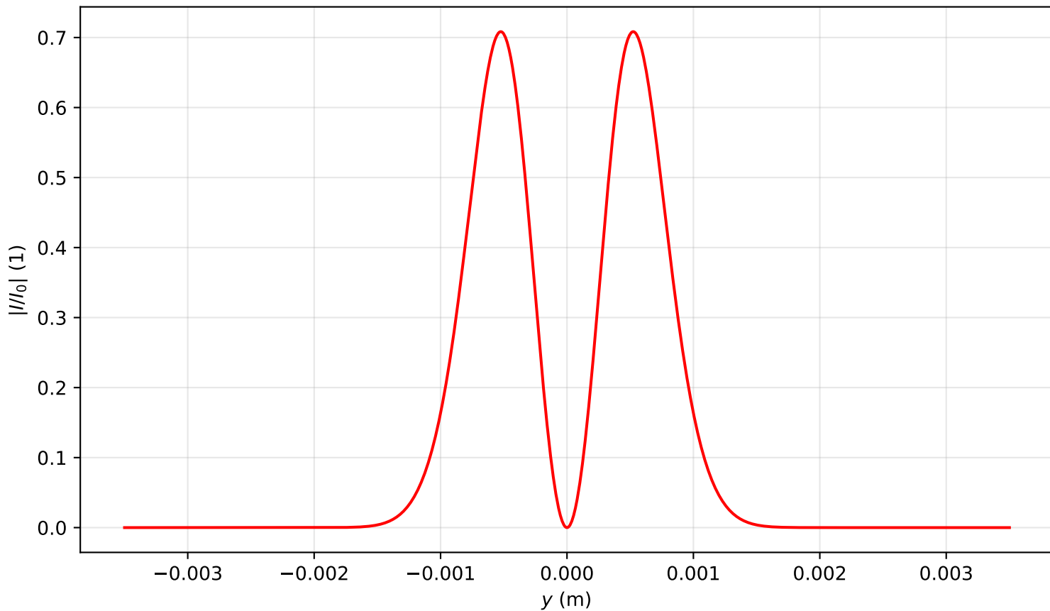
Intensity profile I(x=0, y, z=0.637)/I_0 , P_{in}=0.5P_{cr} , artificial time
